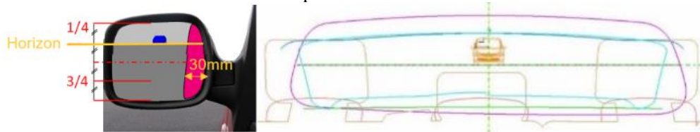
Figure 4. The mirrors' configuration
